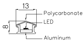
LED BAR (DETAIL)
